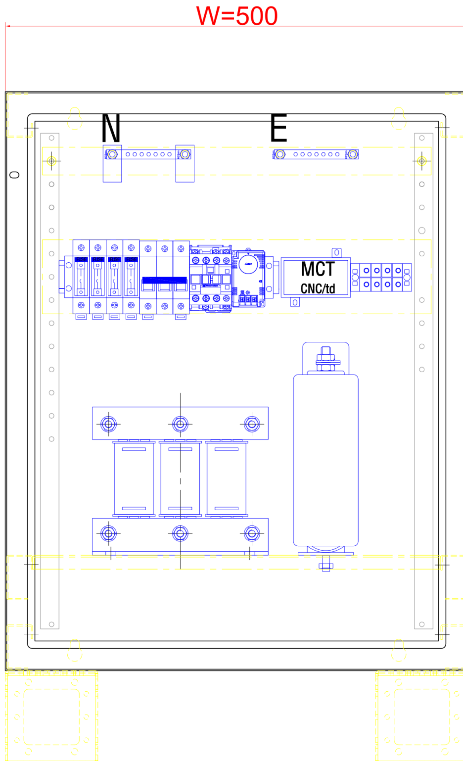
INSIDE VIEW
