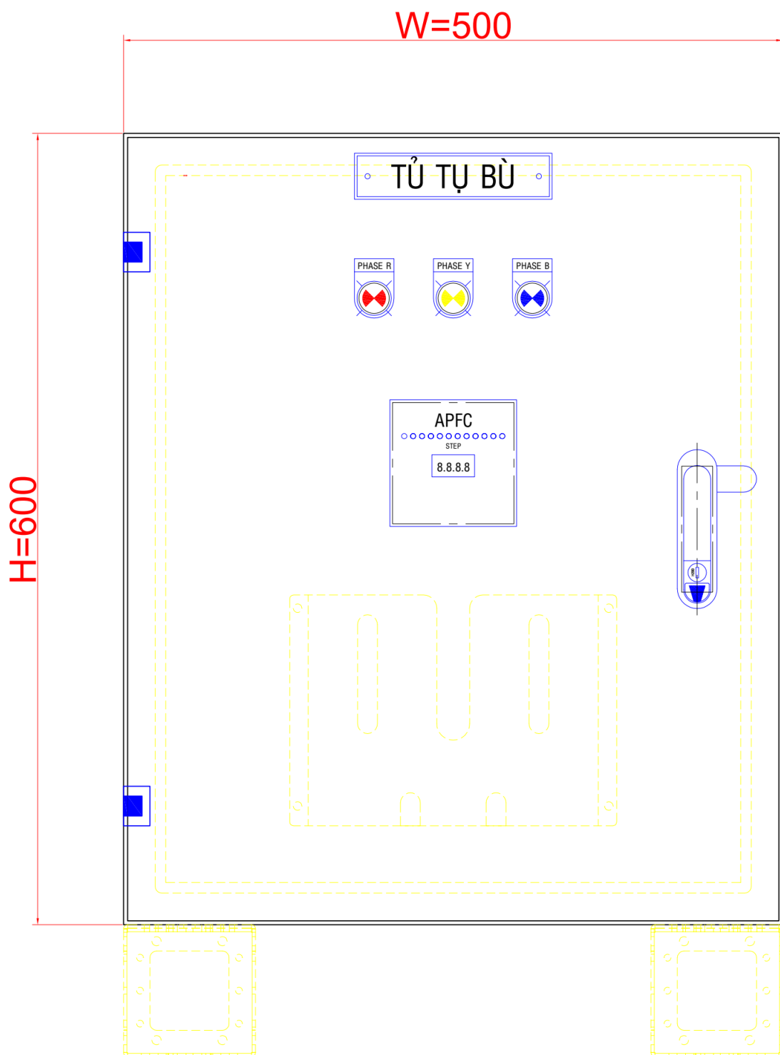
FRONT VIEW
